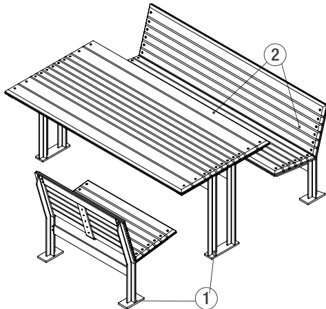
KNIGHT TABLE ENSEMBLE, BACKED WITH ADA OPTION, FSC® 100% CUMARU HARDWOOD SLATS
