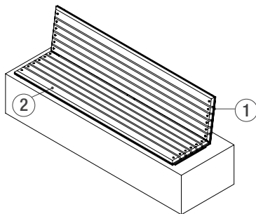
KNIGHT BENCH, 6-FOOT, BACKED, WALL-TOP MOUNT
