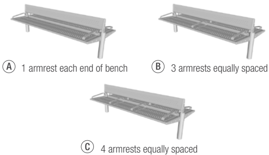
FIG 2: ARMREST LOCATIONS
