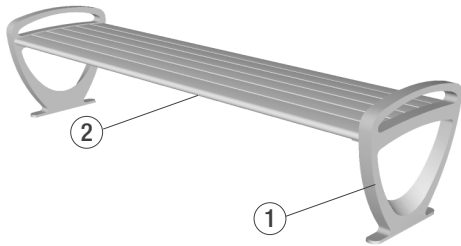
FIG 2: 72" BACKLESS BENCH, ALUMINUM SLATS
