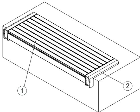
FIG 2: VECTOR WALL-TOP MOUNT BENCH, 2-FOOT, BACKLESS
