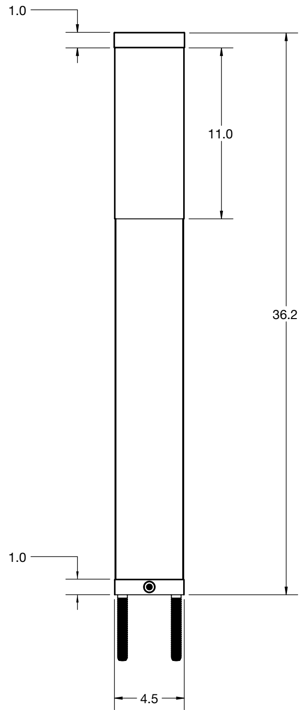
SIDE VIEW
