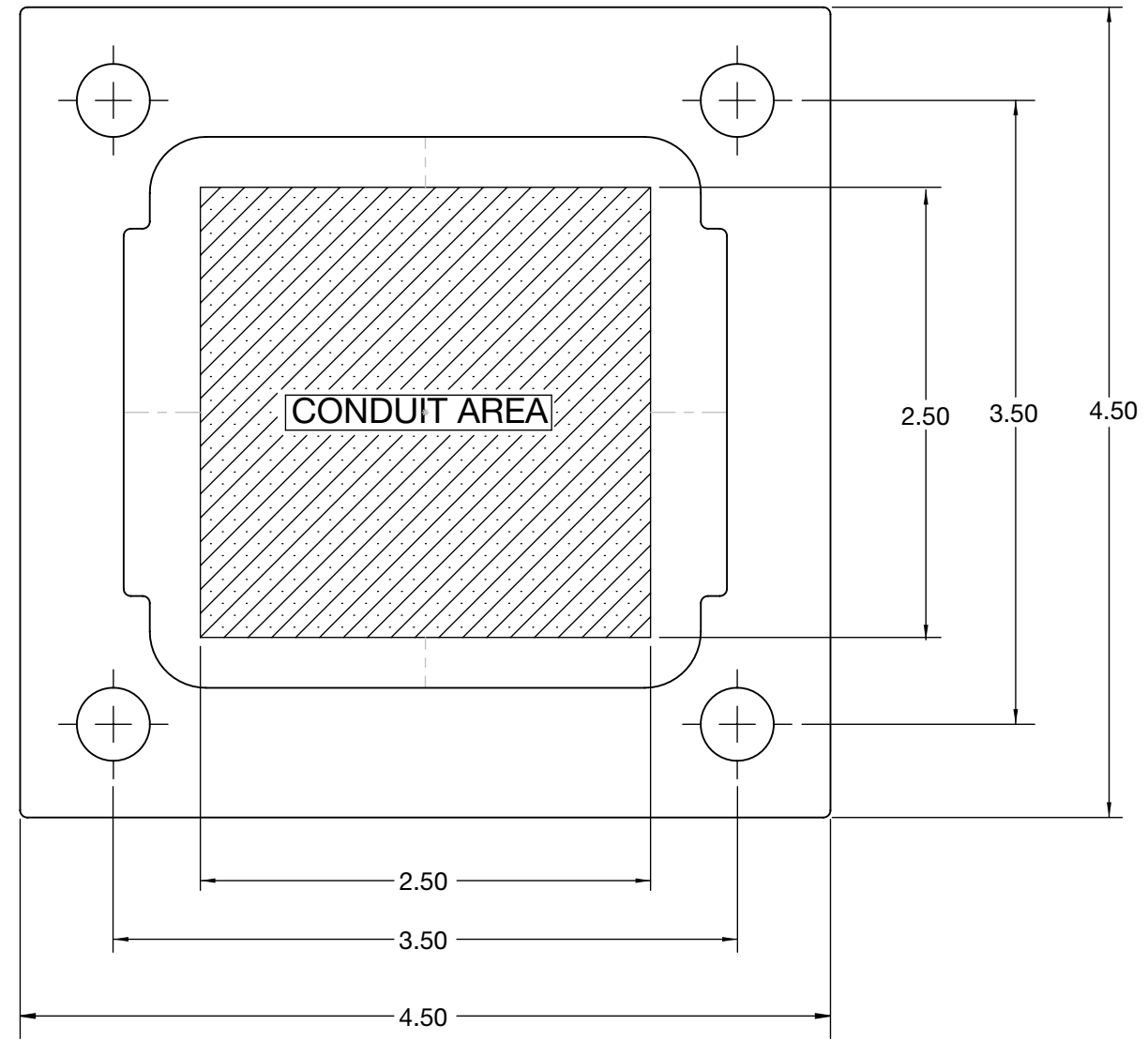
BASE PLATE MOUNTING DETAIL
