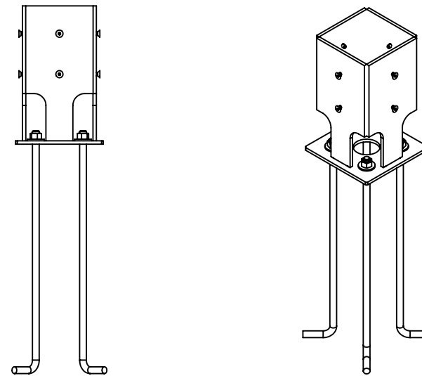
BASE PLATE & J-BOLT ANCHORS
