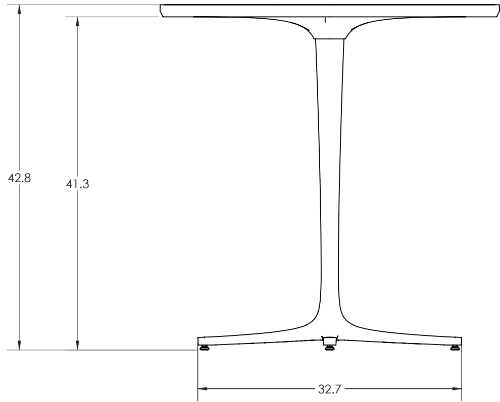
FRONT VIEW
