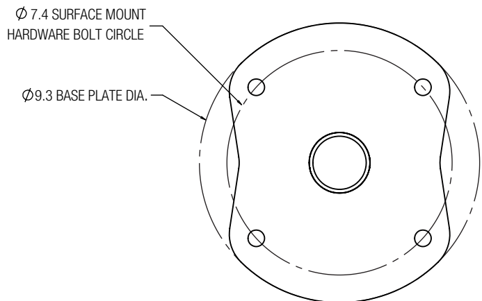
BASE PLATE
